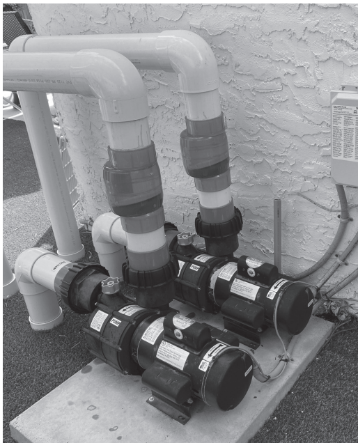
Figure 8 Check Valves Installed for a Package D ( three jet & 2 pump system)
