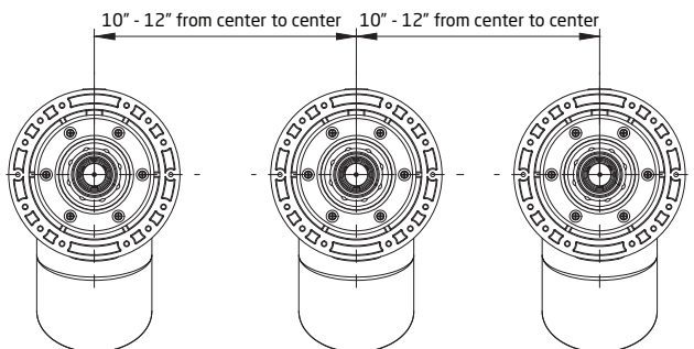
Figure 1A Three Jet (10" - 12" from center to center)
