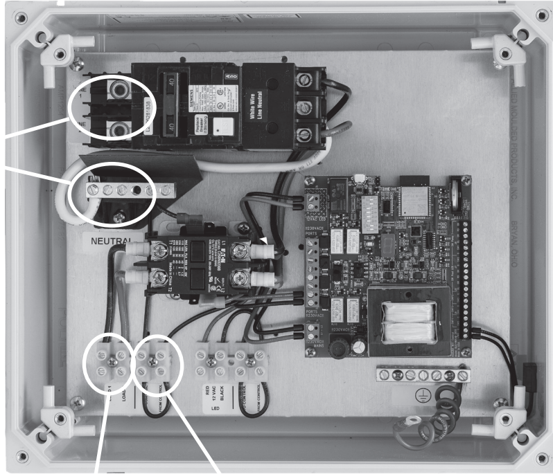
Figure 17 Control Box Wiring
