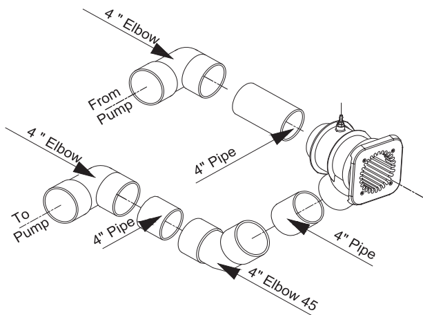
Figure 5 BaduStream Single Housing Installation
